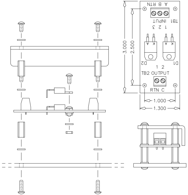
C-SUPPLY BOARD MOUNTED ON PANEL (WITH COVER REMOVED) 1:2 SCALE
